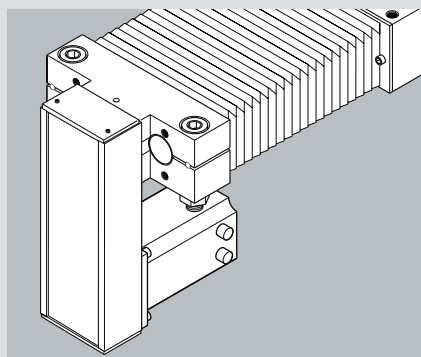
Motor attachment via timing belt side drive
